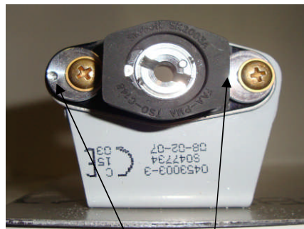
SK2003-AW5 CamWashers set at full left of center position
