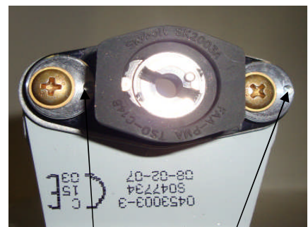
SK2003-AW5 CamWashers set at full right of center position
